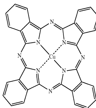
CuPc
