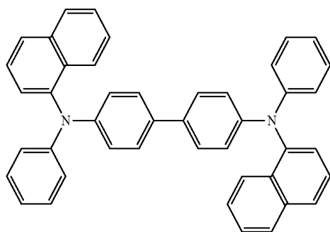
NPD
